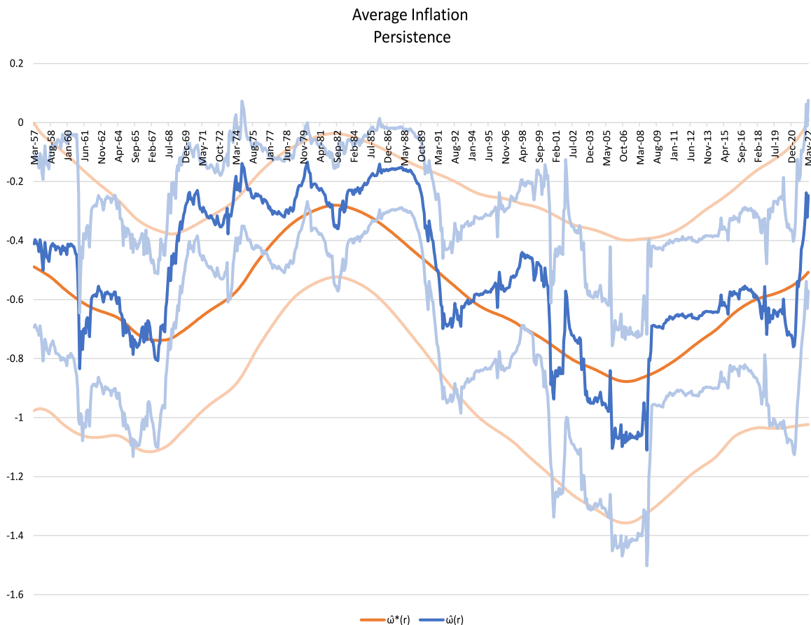
Fig. 2. The potential bias using different methods.
