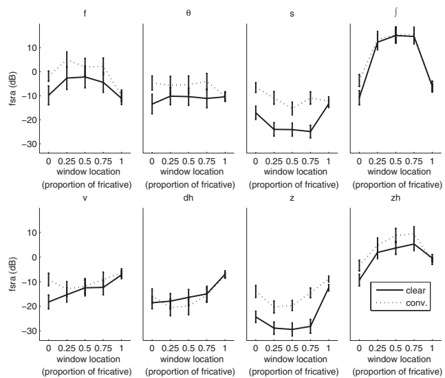
FIG. 9. Mean (and standard error) frequency-specific relative amplitude (FSRA) values as a function of fricative and style.
